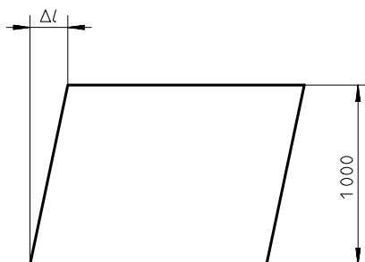
Figure 1 — Rectangularity
